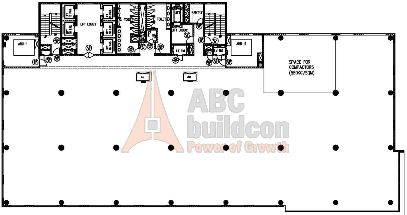
BLOCK THREE-THIRD FLOOR PLAN
