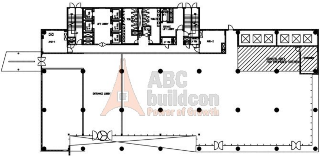
BLOCK THREE - GROUND FLOOR PLAN
